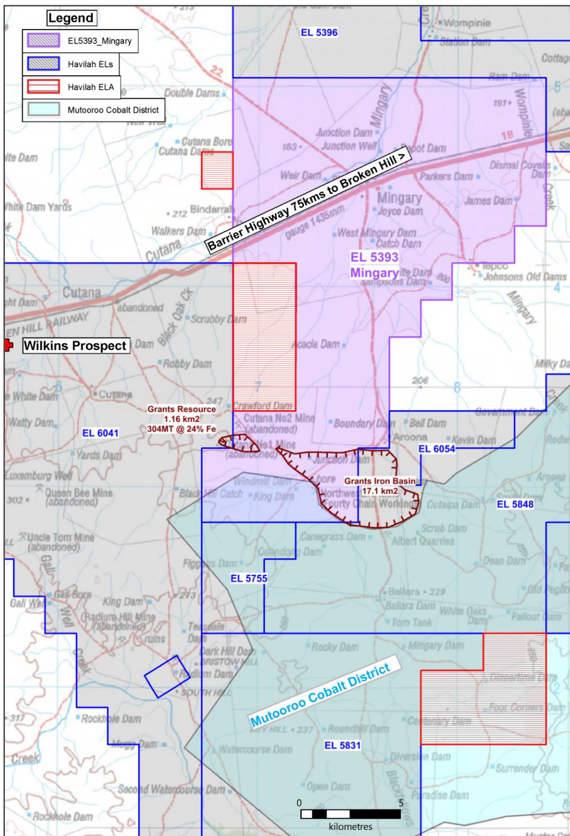
Figure 1 – Location EL 5393 in relation to Grants Iron Ore Deposit, Grants Iron Ore Basin and the Mutooroo Cobalt District
